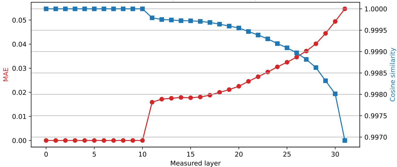
Mistral-7B-Instruct-v0.3 | Quantized layer 10 | float16 → int4
