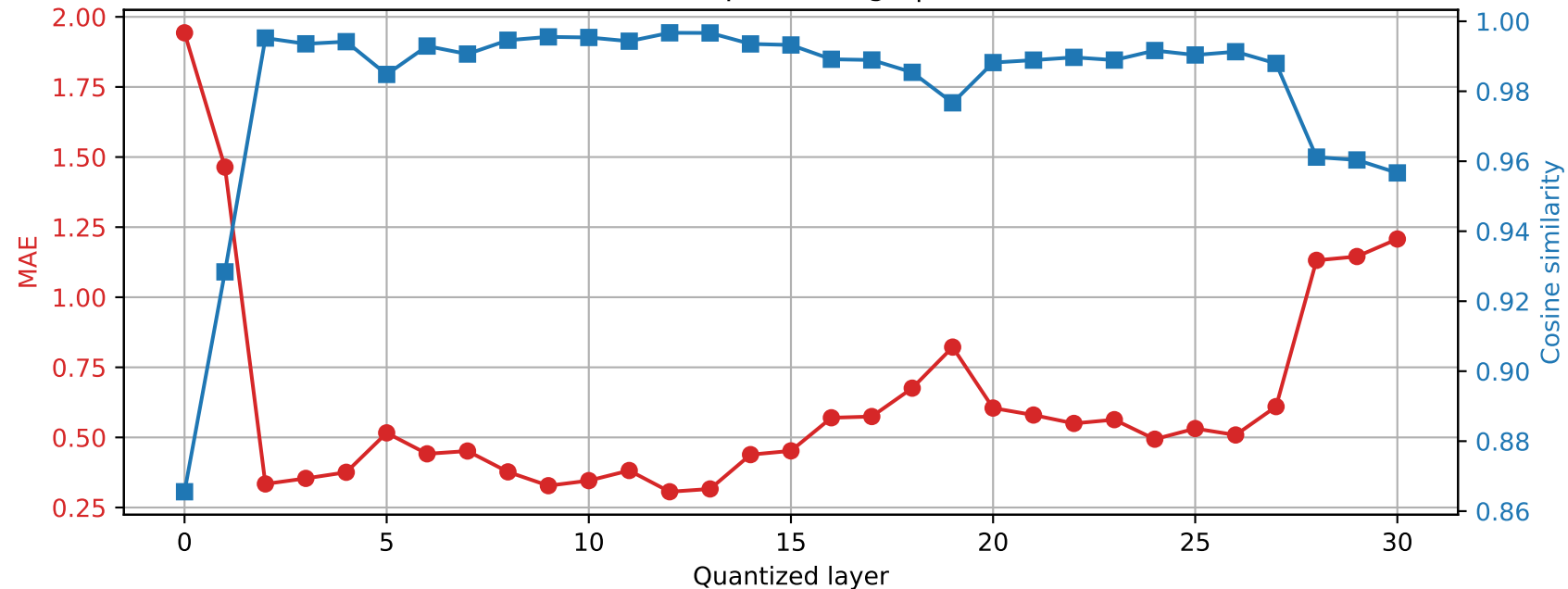
Mistral-7B-Instruct-v0.3 | Prompt 4 Final RMSNorm output damage | float16 \rightarrow int4
