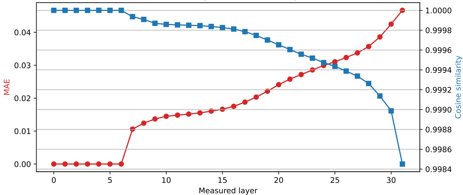
Mistral-7B-Instruct-v0.3 | Quantized layer 6 | float16 → int4
