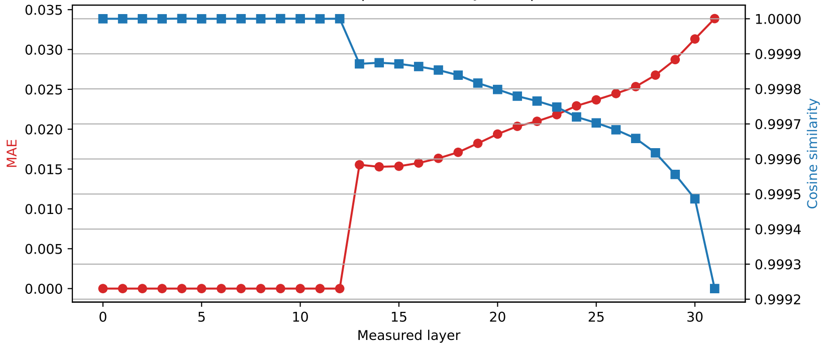
Mistral-7B-Instruct-v0.3 | Quantized layer 12 | float16 \rightarrow int4
