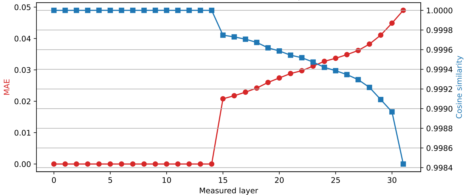
Mistral-7B-Instruct-v0.3 | Quantized layer 14 | float16 \rightarrow int4
