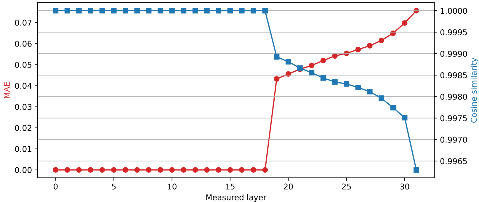
Mistral-7B-Instruct-v0.3 | Quantized layer 18 | float16 → int4
