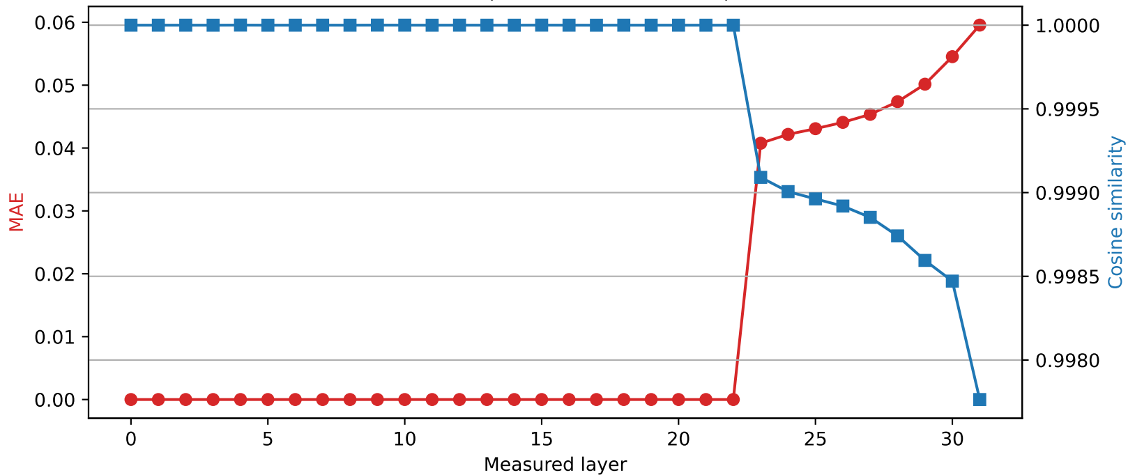
Mistral-7B-Instruct-v0.3 | Quantized layer 22 | float16 → int4
