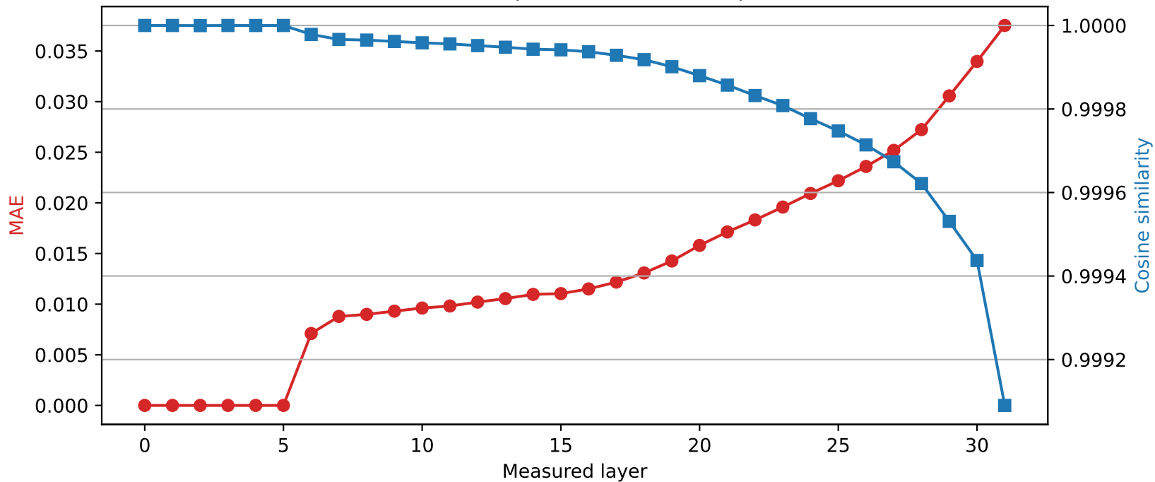
Mistral-7B-Instruct-v0.3 | Quantized layer 5 | float16 → int2
