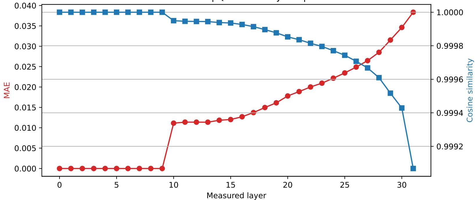
Mistral-7B-Instruct-v0.3 | Quantized layer 9 | float16 \rightarrow int2
