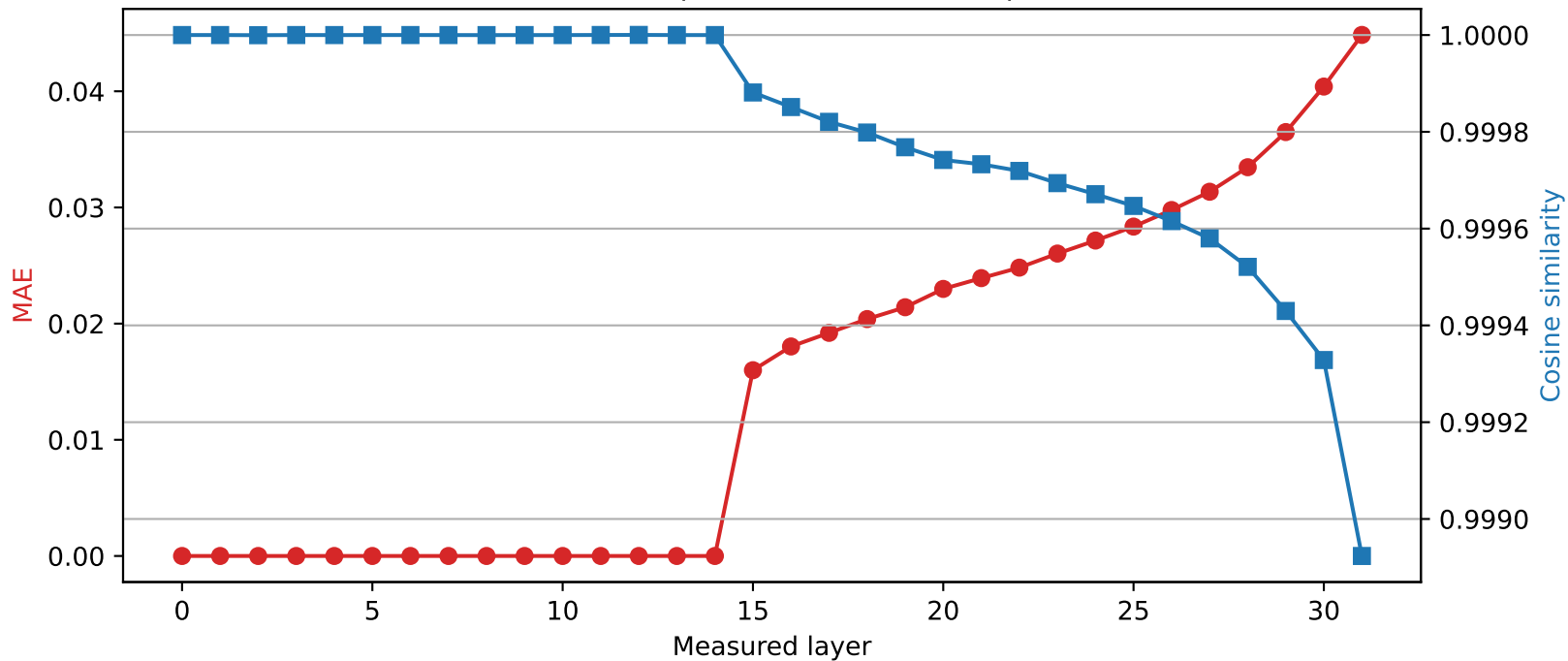
Mistral-7B-Instruct-v0.3 | Quantized layer 14 | float16 → int2
