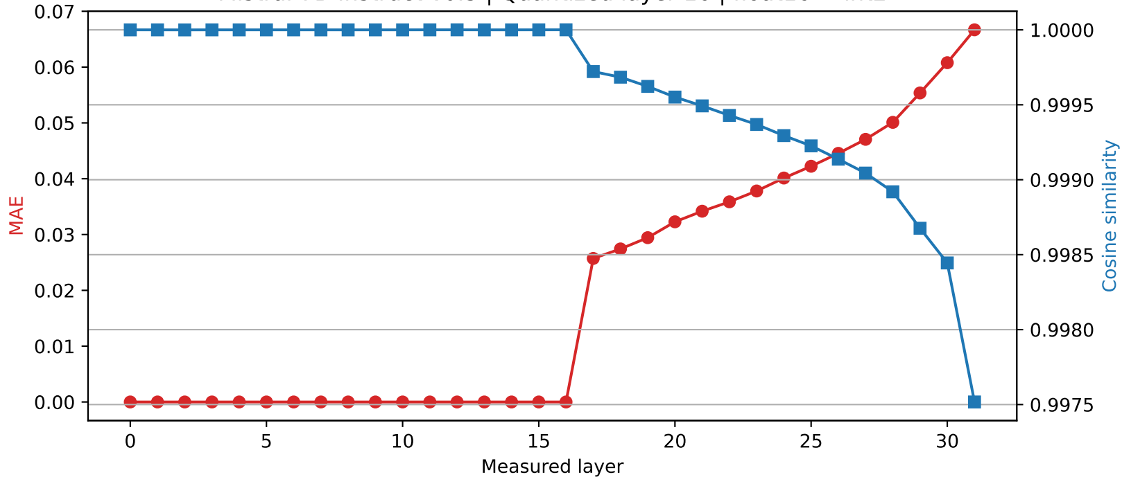
Mistral-7B-Instruct-v0.3 | Quantized layer 16 | float16 \rightarrow int2
