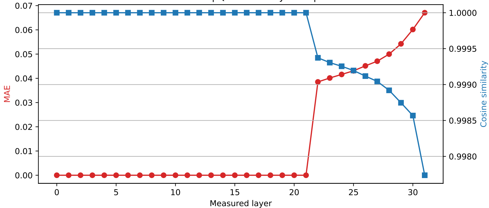
Mistral-7B-Instruct-v0.3 | Quantized layer 21 | float16 \rightarrow int2
