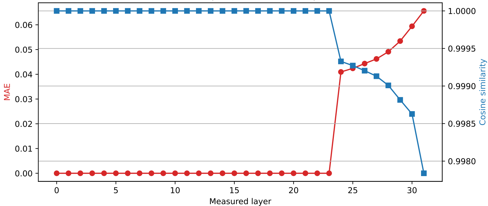
Mistral-7B-Instruct-v0.3 | Quantized layer 23 | float16 \rightarrow int2
