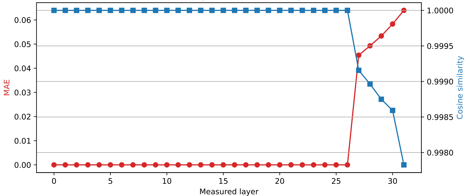
Mistral-7B-Instruct-v0.3 | Quantized layer 26 | float16 \rightarrow int2
