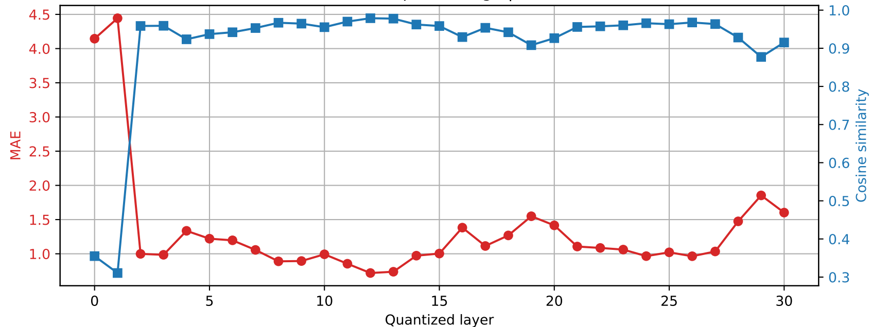
Mistral-7B-Instruct-v0.3 | Prompt 1 Final RMSNorm output damage | float16 \rightarrow int2
