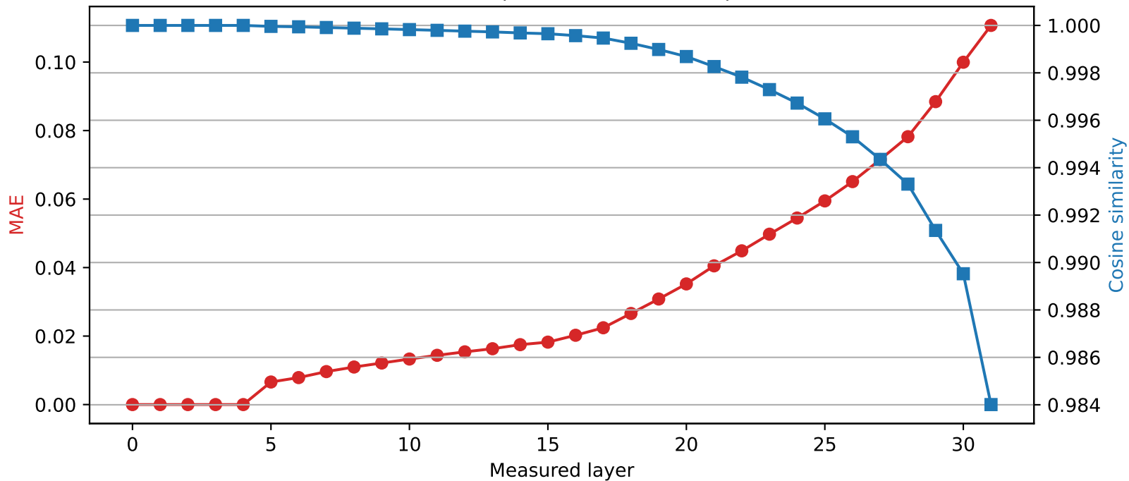
Mistral-7B-Instruct-v0.3 | Quantized layer 4 | float16 \rightarrow int2
