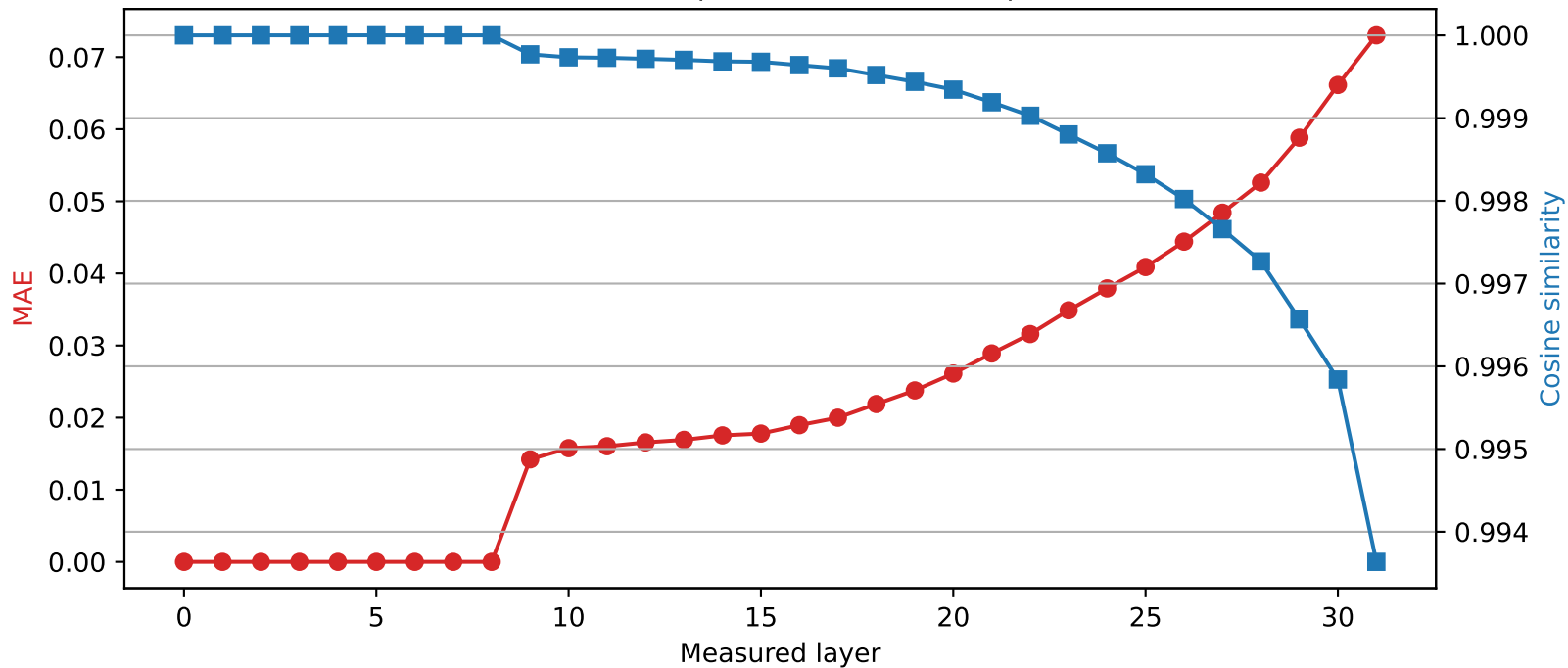
Mistral-7B-Instruct-v0.3 | Quantized layer 8 | float16 → int2
