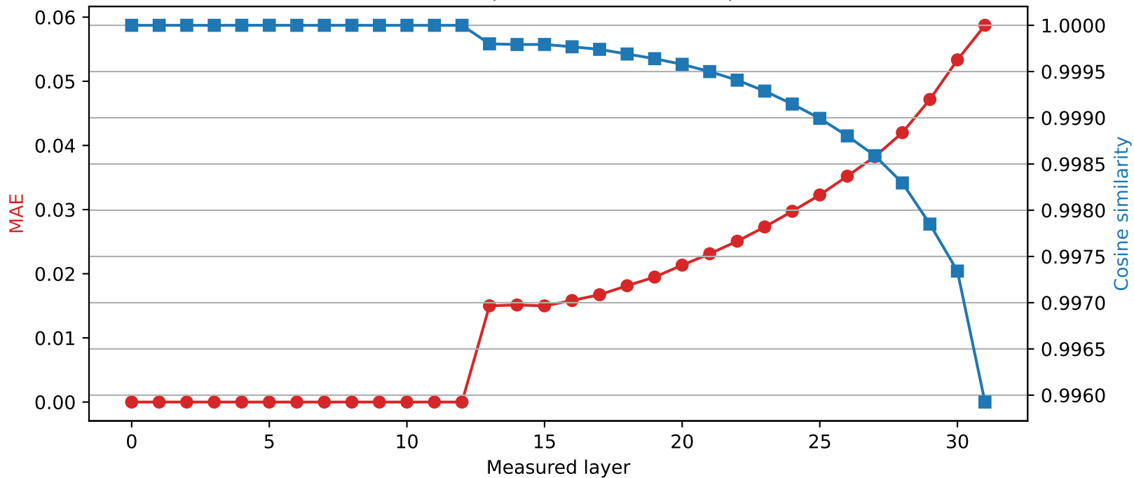
Mistral-7B-Instruct-v0.3 | Quantized layer 12 | float16 \rightarrow int2
