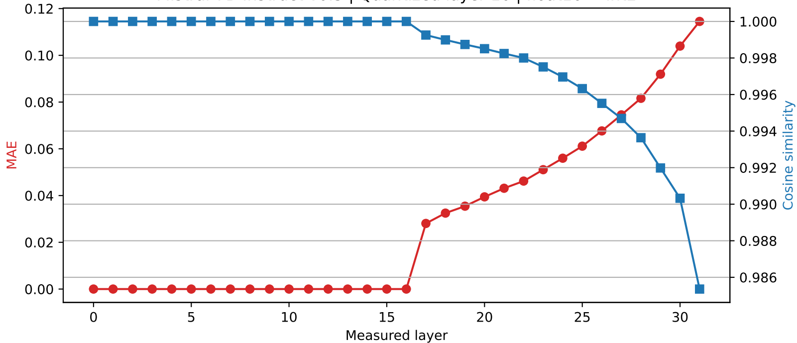
Mistral-7B-Instruct-v0.3 | Quantized layer 16 | float16 → int2
