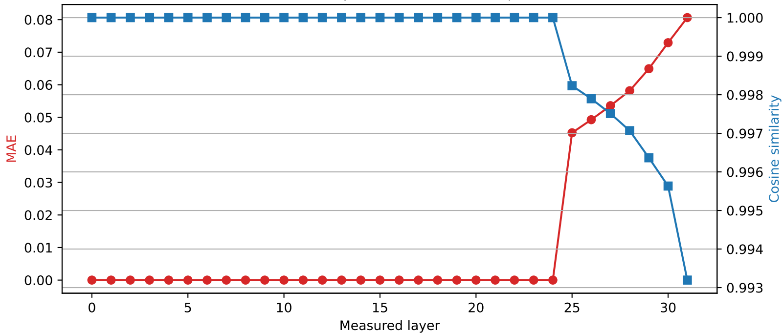
Mistral-7B-Instruct-v0.3 | Quantized layer 24 | float16 \rightarrow int2
