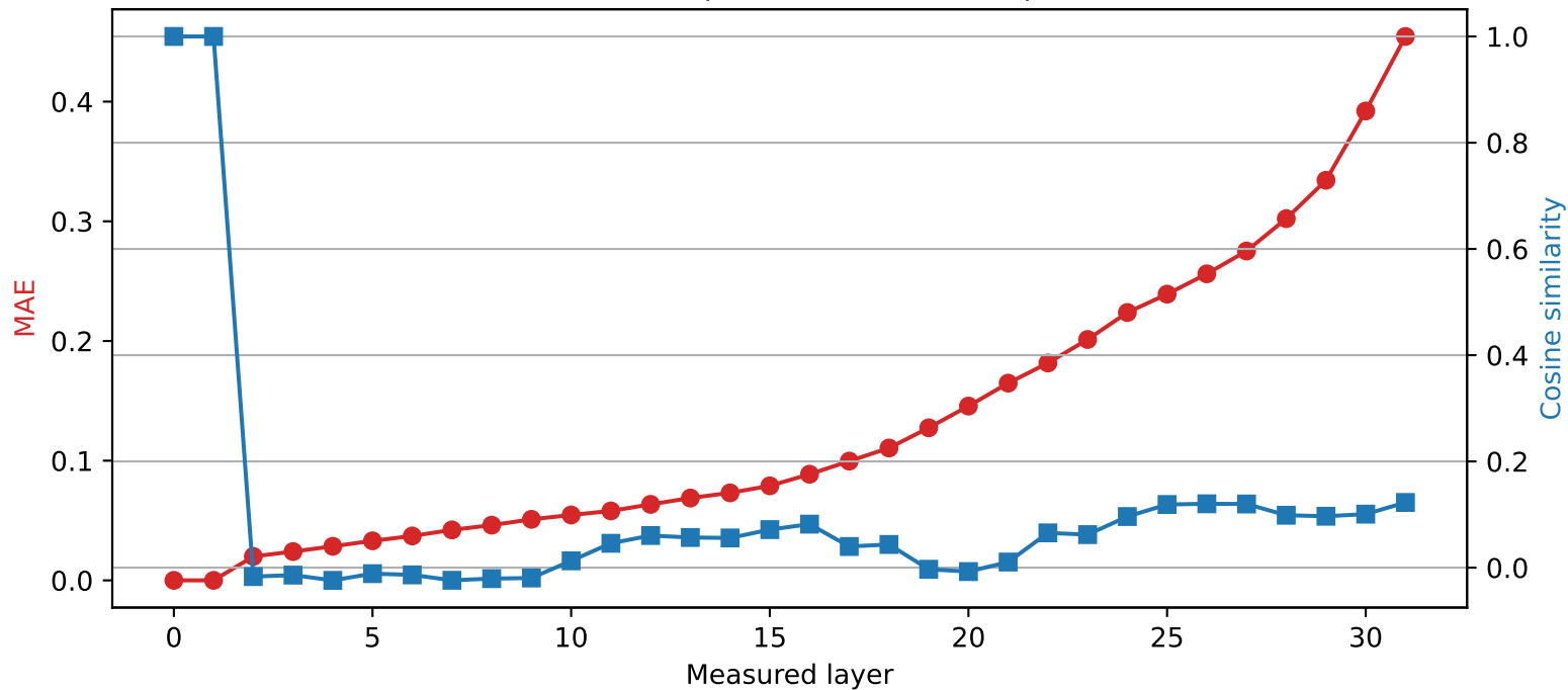
Mistral-7B-Instruct-v0.3 | Quantized layer 1 | float16 → int2
