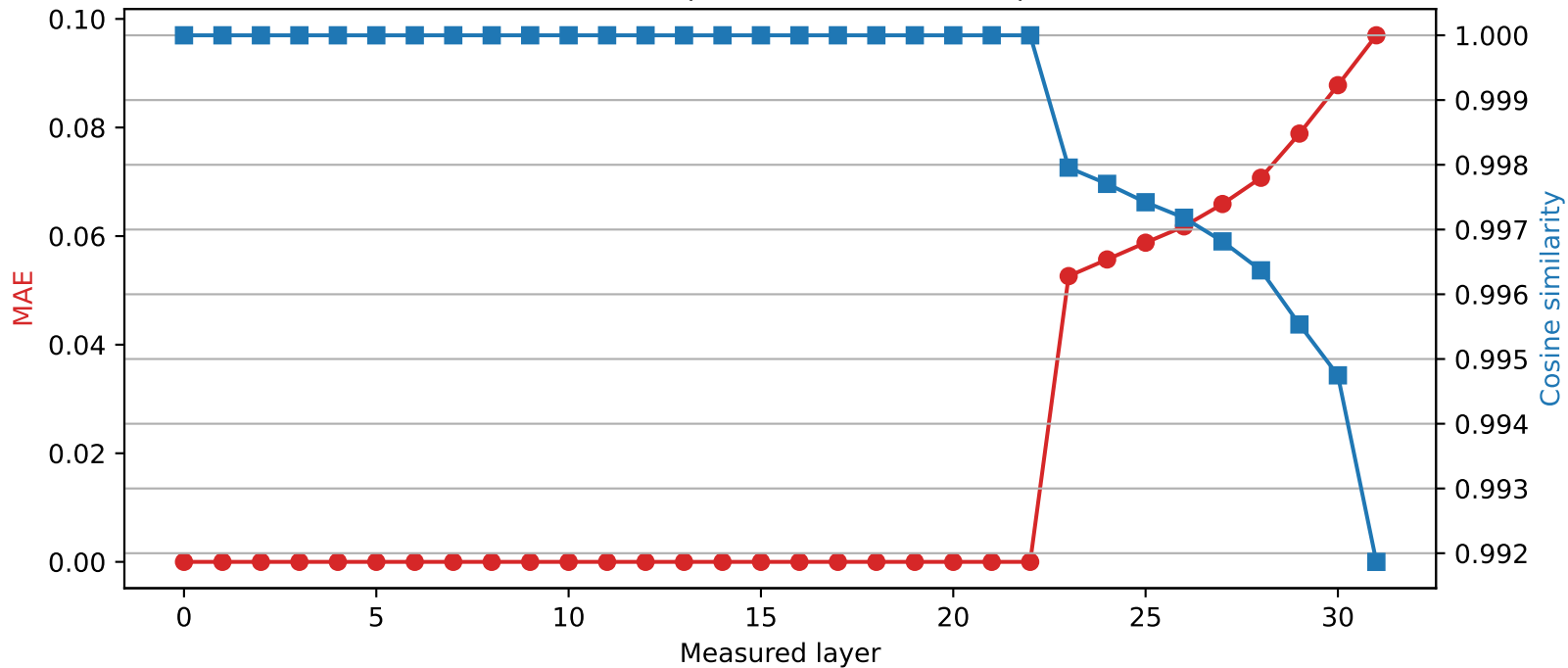
Mistral-7B-Instruct-v0.3 | Quantized layer 22 | float16 \rightarrow int2
