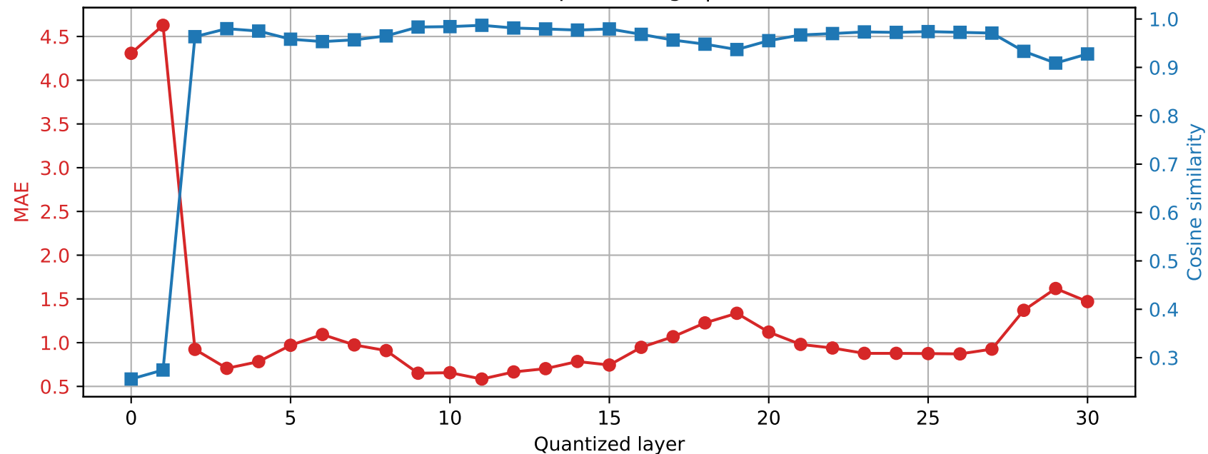
Mistral-7B-Instruct-v0.3 | Prompt 3 Final RMSNorm output damage | float16 \rightarrow int2
