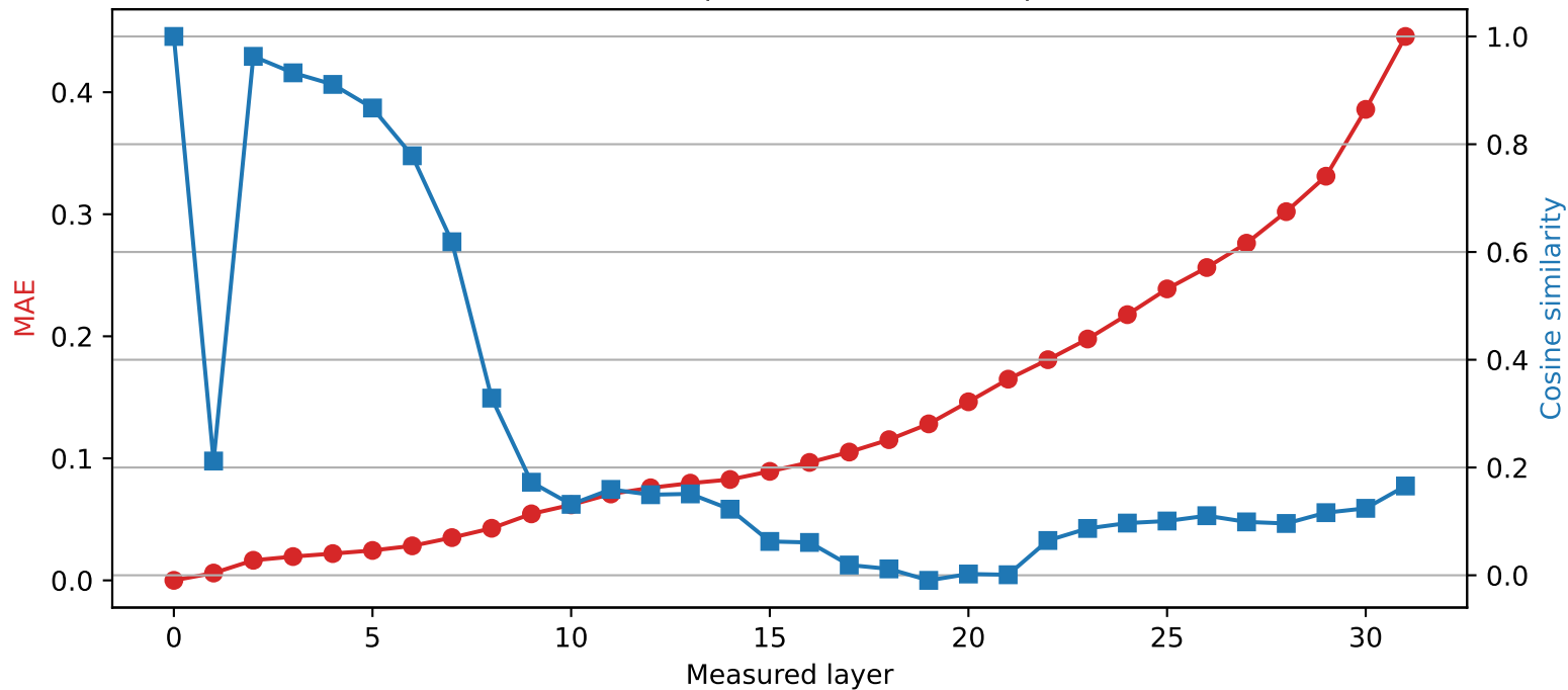
Mistral-7B-Instruct-v0.3 | Quantized layer 0 | float16 \rightarrow int2
