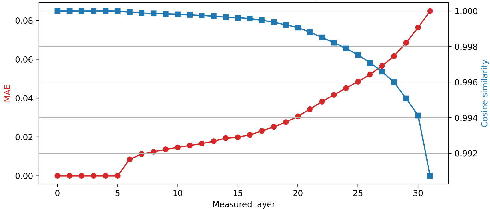
Mistral-7B-Instruct-v0.3 | Quantized layer 5 | float16 \rightarrow int2
