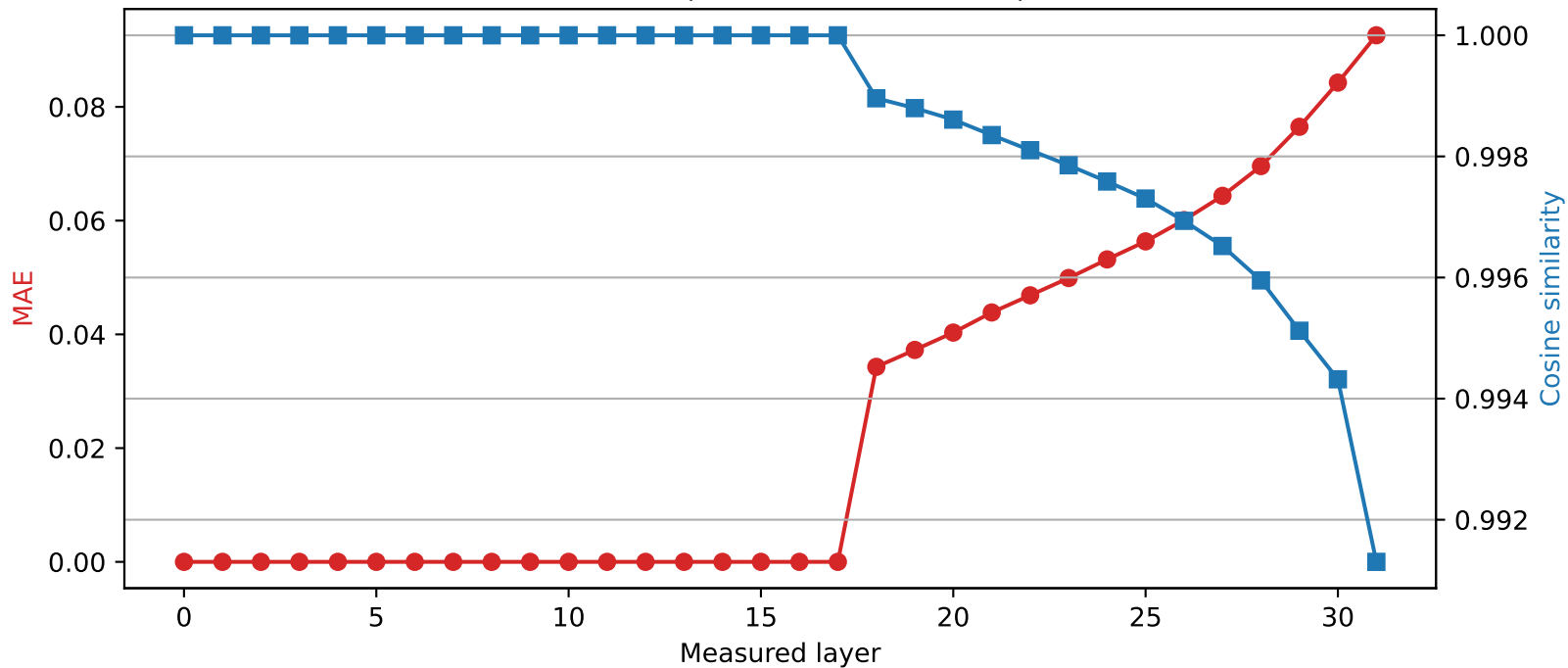
Mistral-7B-Instruct-v0.3 | Quantized layer 17 | float16 → int2
