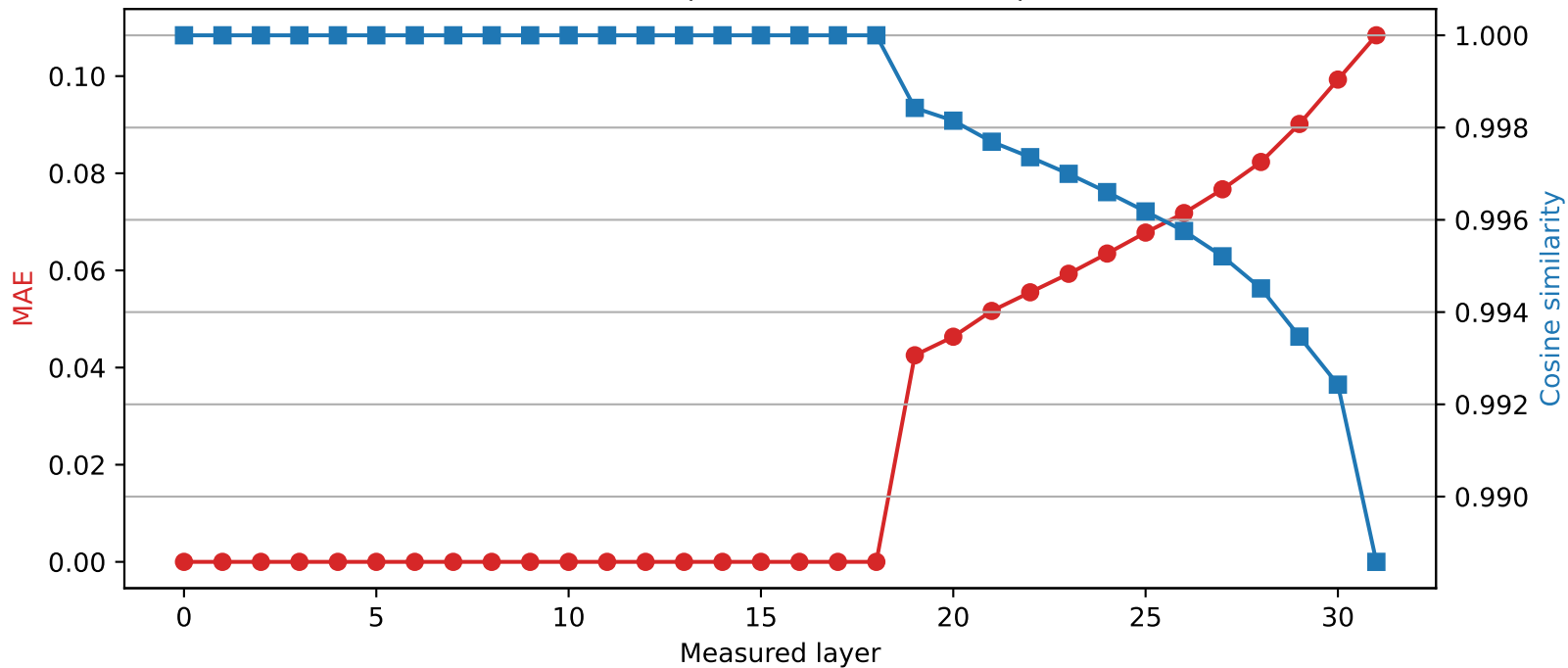
Mistral-7B-Instruct-v0.3 | Quantized layer 18 | float16 \rightarrow int2
