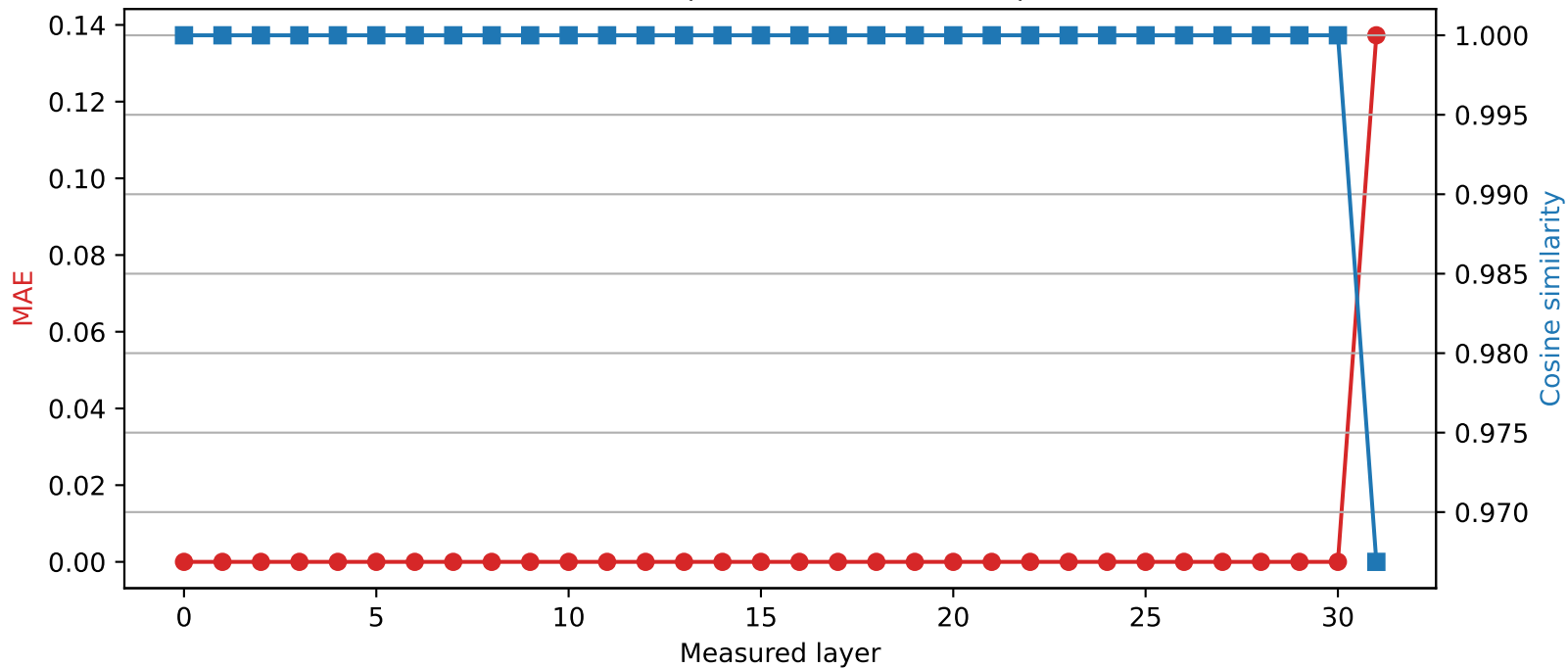
Mistral-7B-Instruct-v0.3 | Quantized layer 30 | float16 \rightarrow int2
