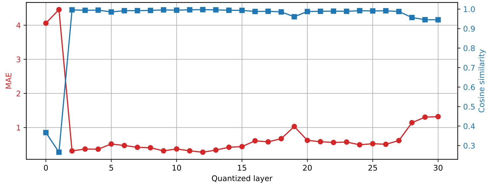
Mistral-7B-Instruct-v0.3 | Prompt 4 Final RMSNorm output damage | float16 \rightarrow int2
