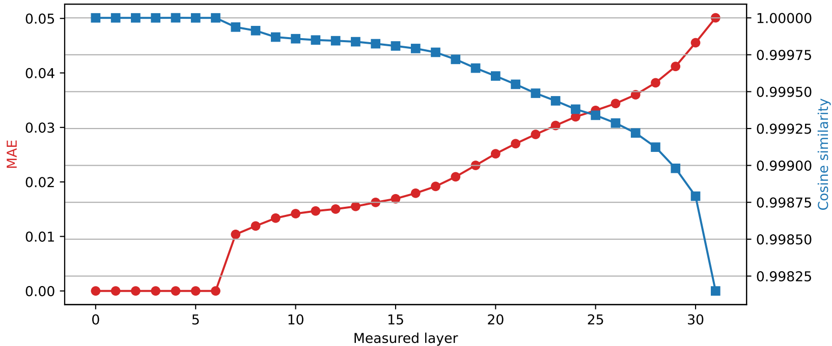
Mistral-7B-Instruct-v0.3 | Quantized layer 6 | float16 → int2
