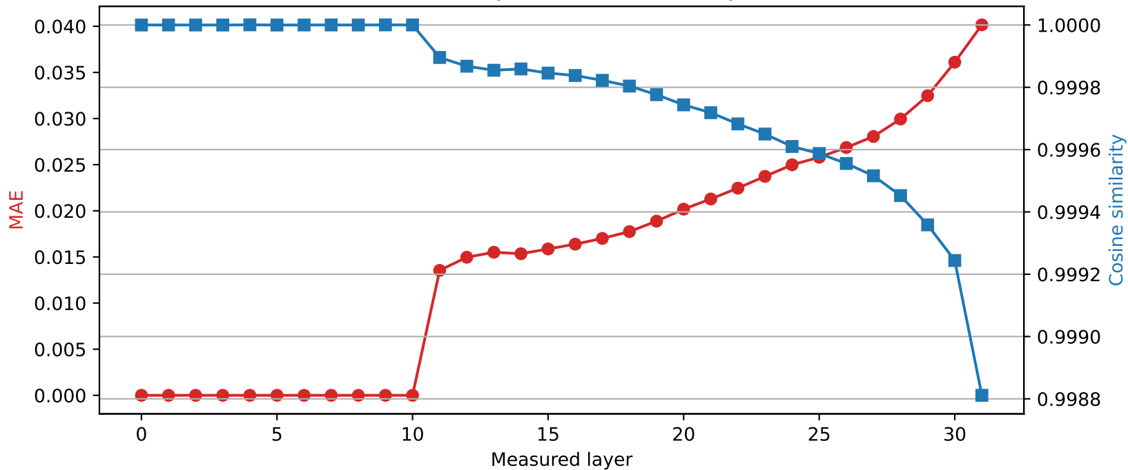
Mistral-7B-Instruct-v0.3 | Quantized layer 10 | float16 \rightarrow int2
