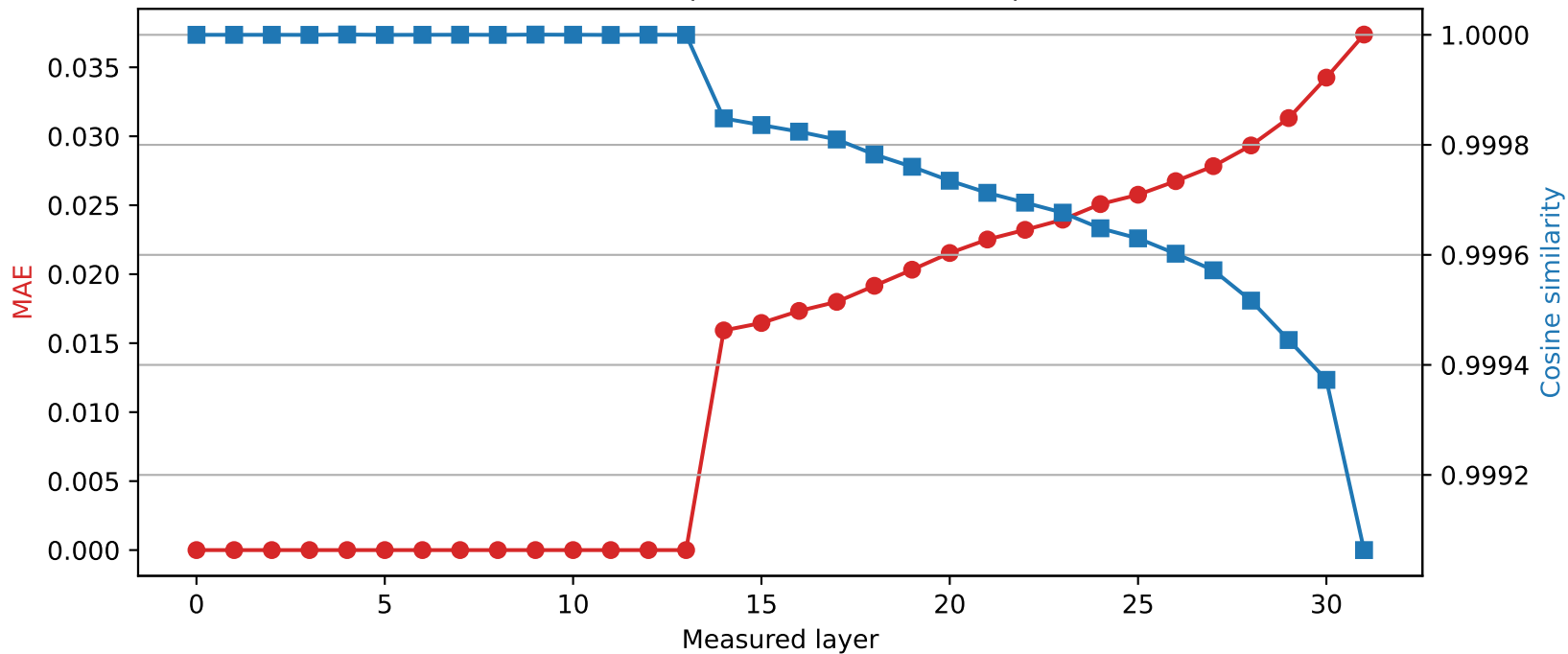
Mistral-7B-Instruct-v0.3 | Quantized layer 13 | float16 \rightarrow int2
