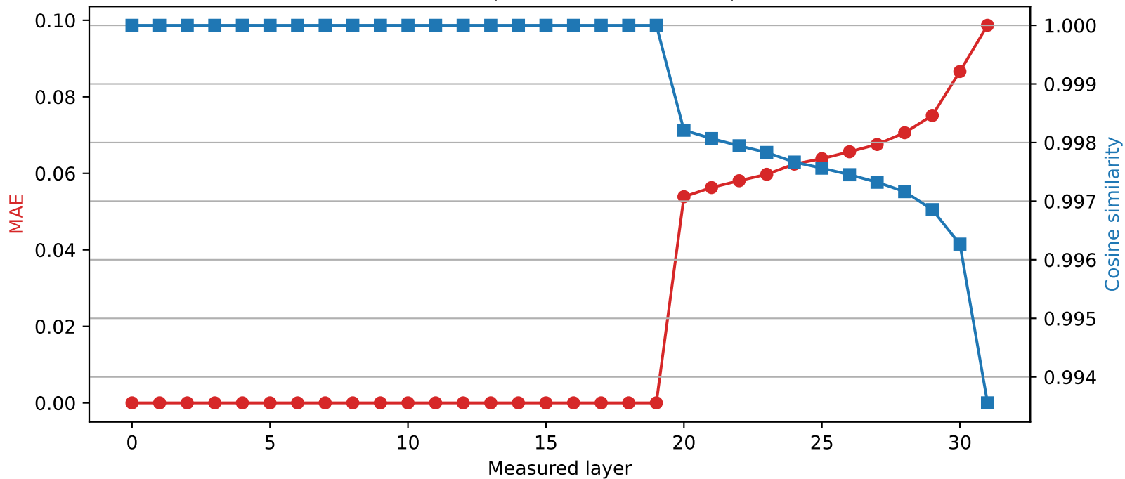
Mistral-7B-Instruct-v0.3 | Quantized layer 19 | float16 \rightarrow int2
