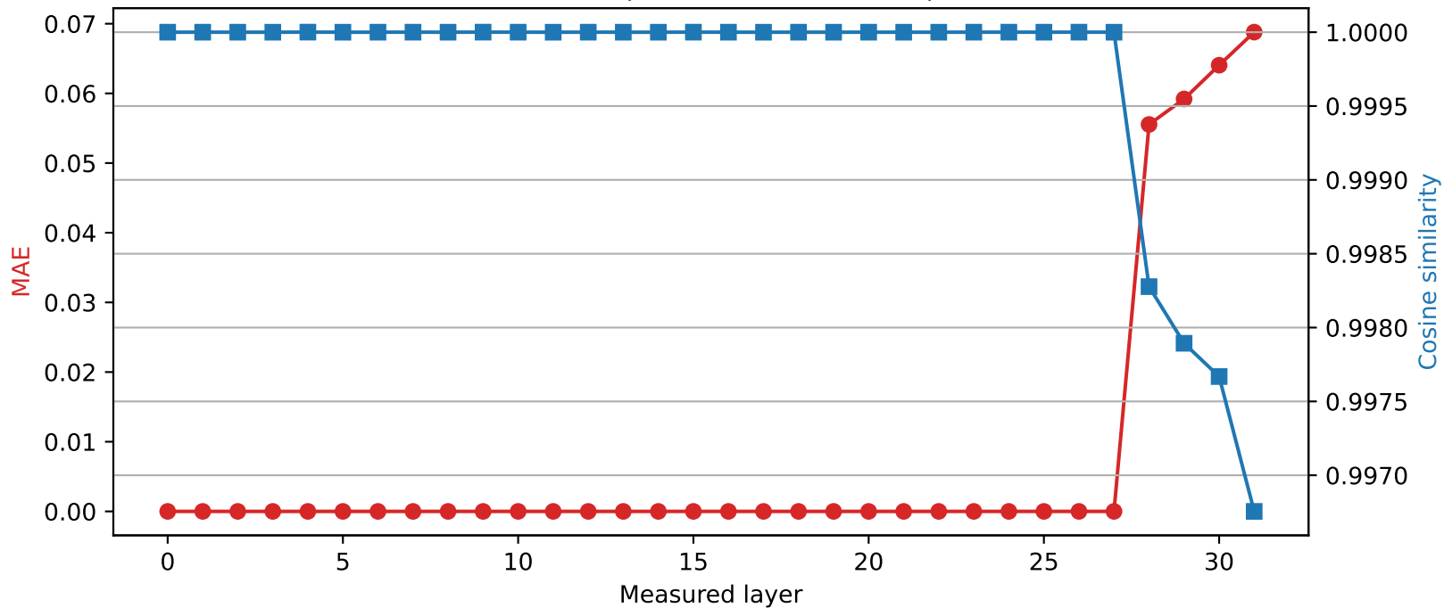
Mistral-7B-Instruct-v0.3 | Quantized layer 27 | float16 \rightarrow int2
