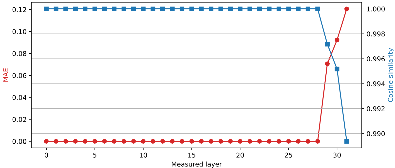
Mistral-7B-Instruct-v0.3 | Quantized layer 28 | float16 \rightarrow int2
