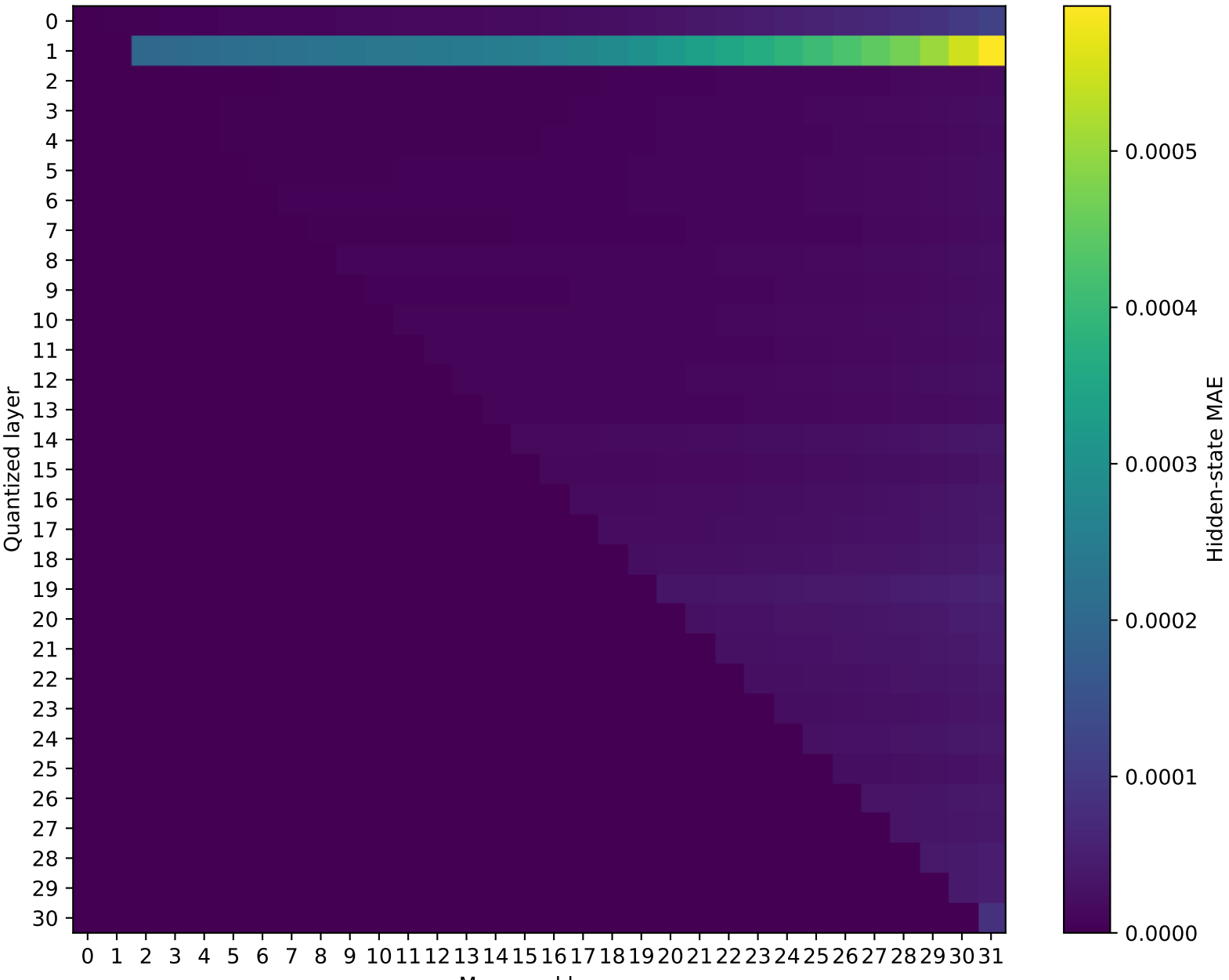
Model: Mistral-7B-Instruct-v0.3 | float32 → int16
