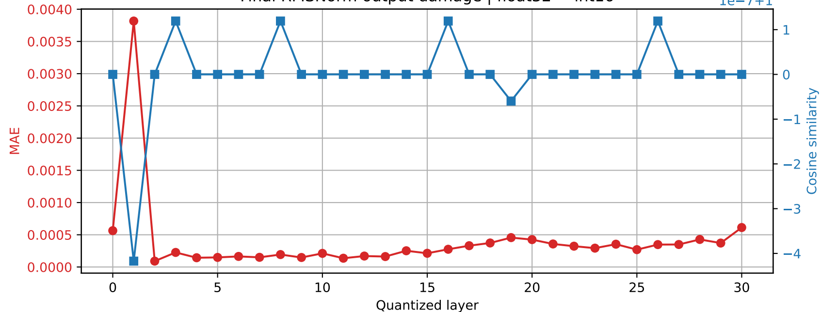
Mistral-7B-Instruct-v0.3 | Prompt 0 Final RMSNorm output damage | float32 \rightarrow int16
