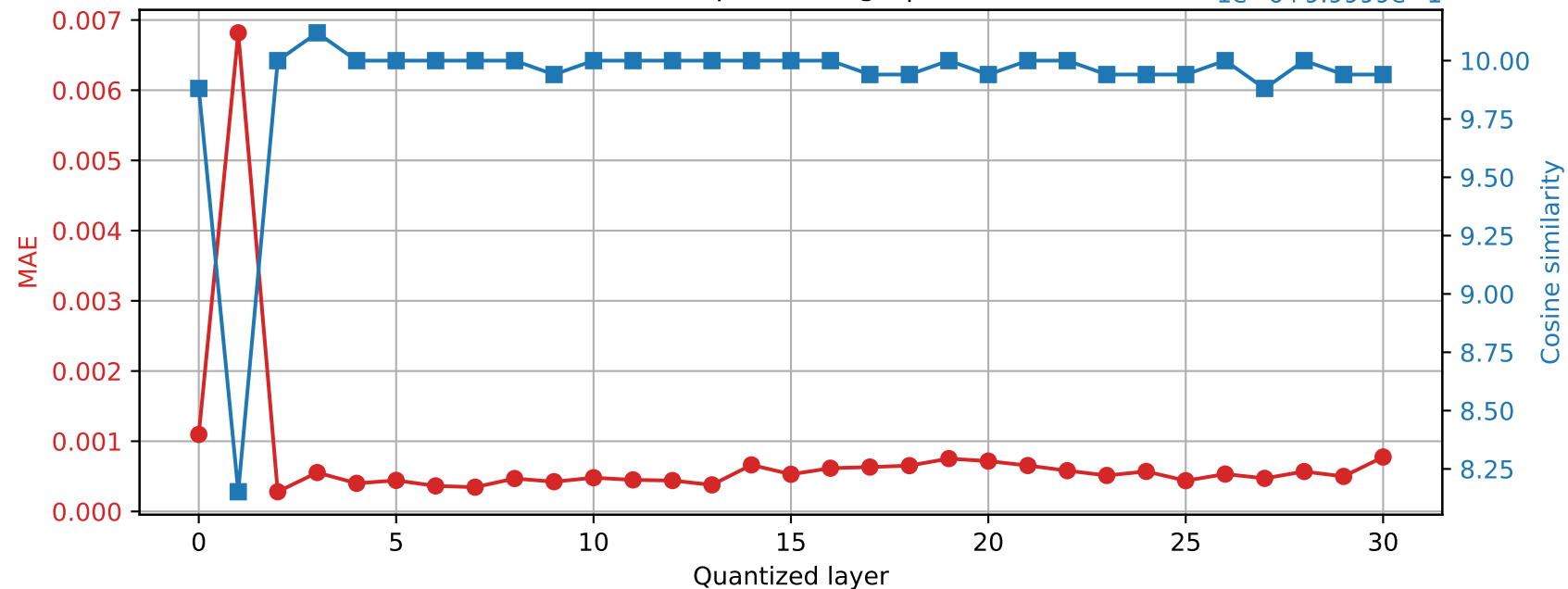
Mistral-7B-Instruct-v0.3 | Prompt 1 Final RMSNorm output damage | float32 → int16
