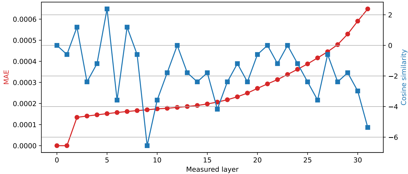
Mistral-7B-Instruct-v0.3 | Quantized layer 1 | float32 \rightarrow int16
