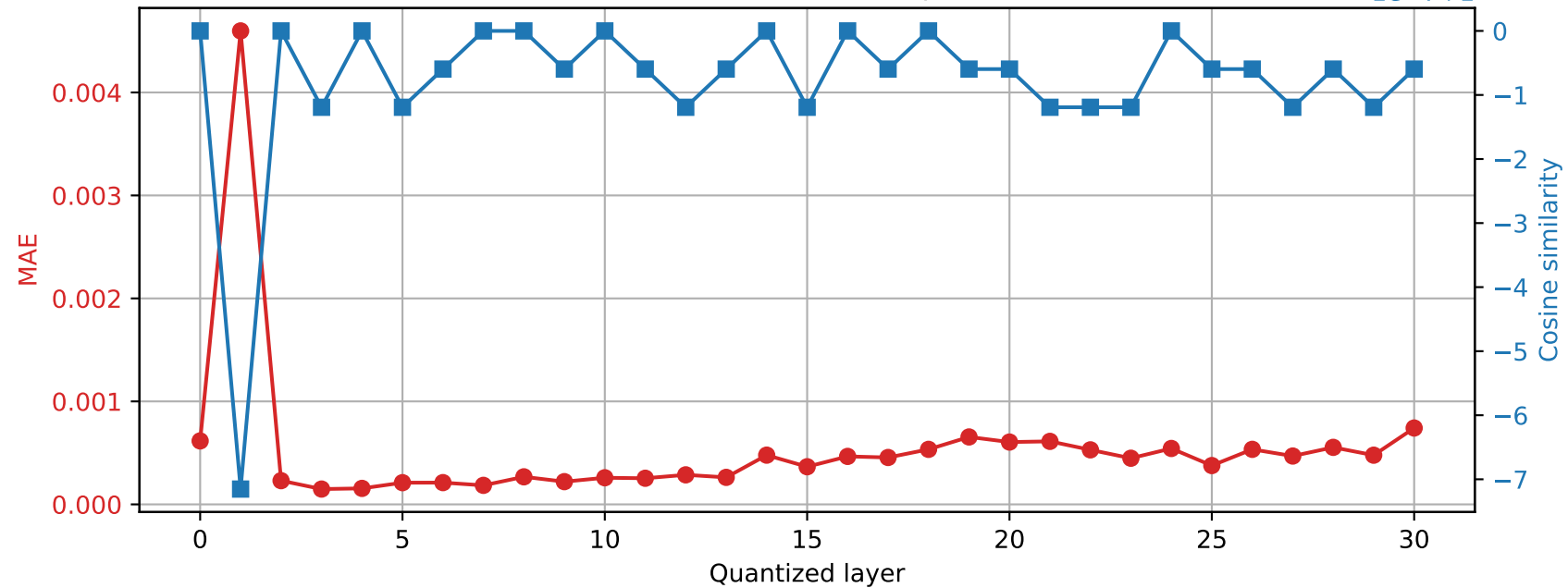
Mistral-7B-Instruct-v0.3 | Prompt 2 Final RMSNorm output damage | float32 → int16
