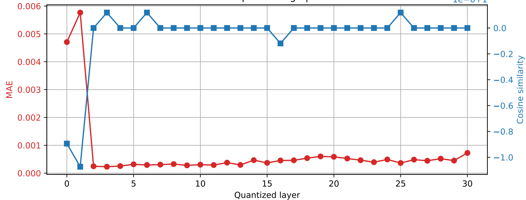
Mistral-7B-Instruct-v0.3 | Prompt 3 Final RMSNorm output damage | float32 \rightarrow int16
