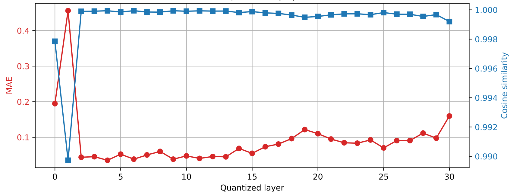
Mistral-7B-Instruct-v0.3 | Prompt 0 Final RMSNorm output damage | float32 → int8
