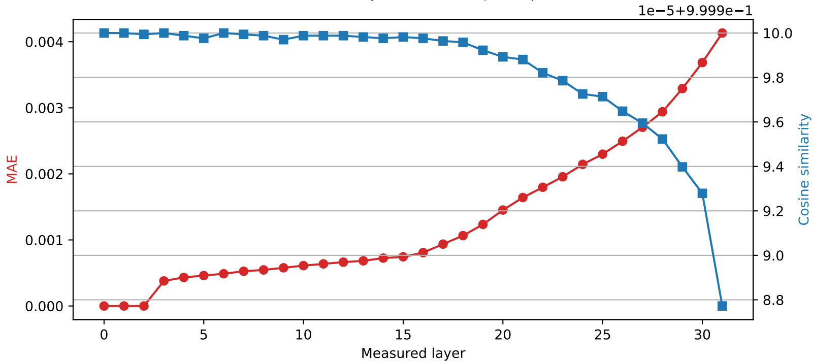
Mistral-7B-Instruct-v0.3 | Quantized layer 2 | float32 → int8
