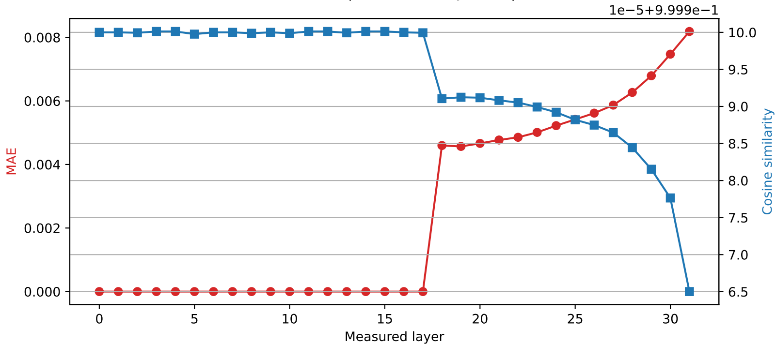
Mistral-7B-Instruct-v0.3 | Quantized layer 17 | float32 \rightarrow int8
