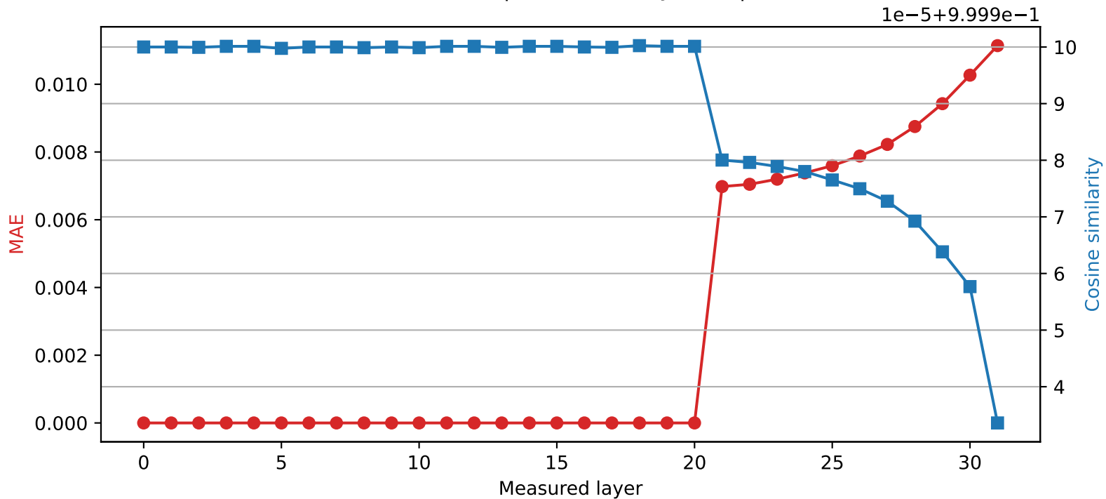
Mistral-7B-Instruct-v0.3 | Quantized layer 20 | float32 \rightarrow int8
