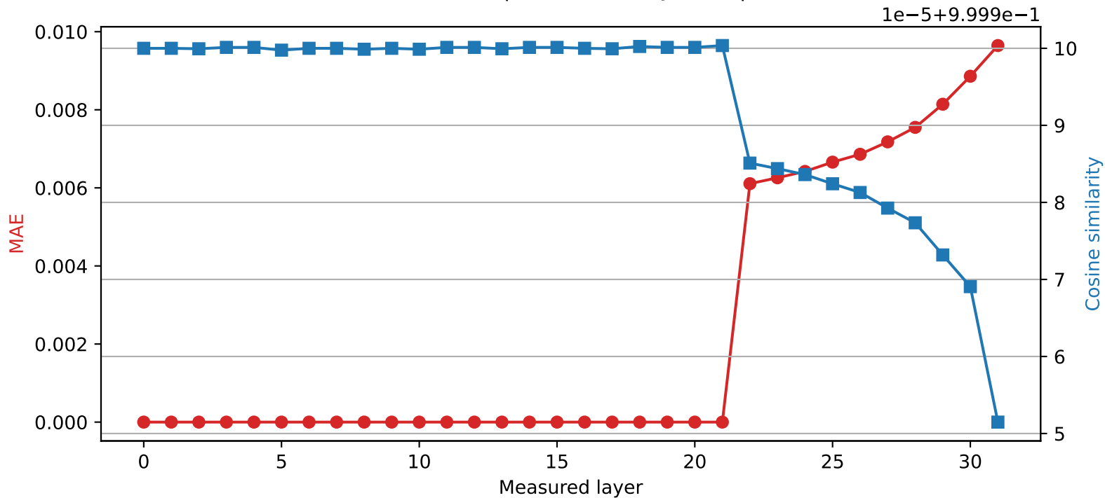
Mistral-7B-Instruct-v0.3 | Quantized layer 21 | float32 \rightarrow int8
