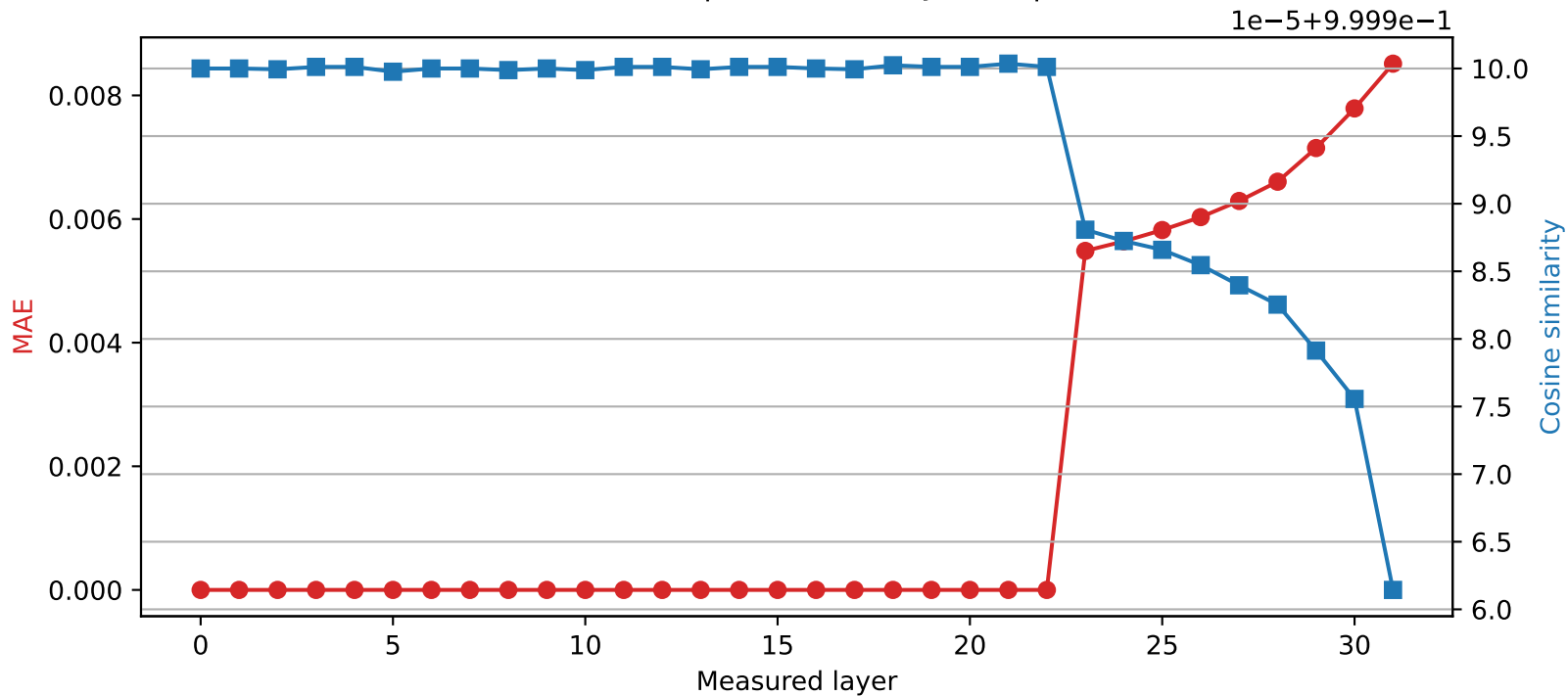
Mistral-7B-Instruct-v0.3 | Quantized layer 22 | float32 → int8
