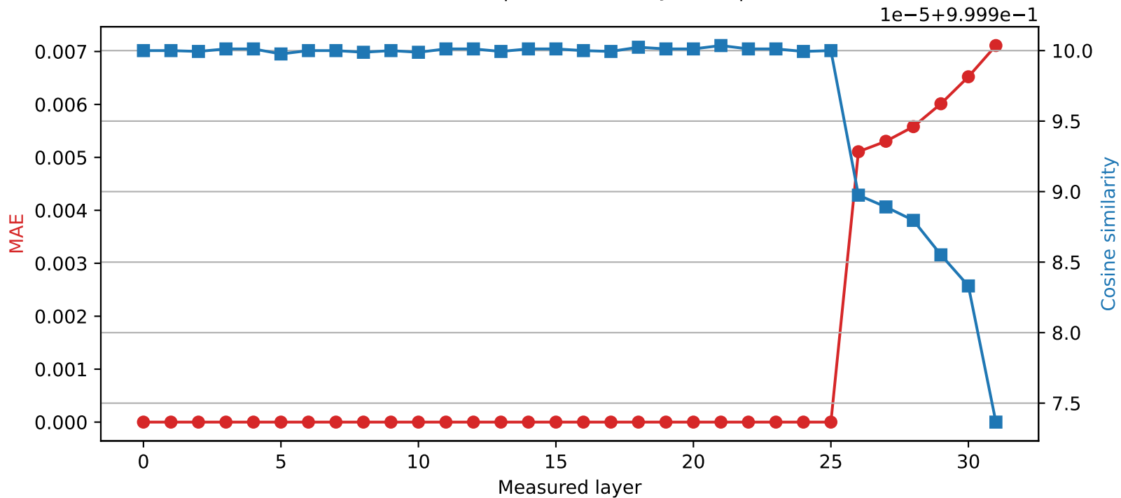
Mistral-7B-Instruct-v0.3 | Quantized layer 25 | float32 → int8
