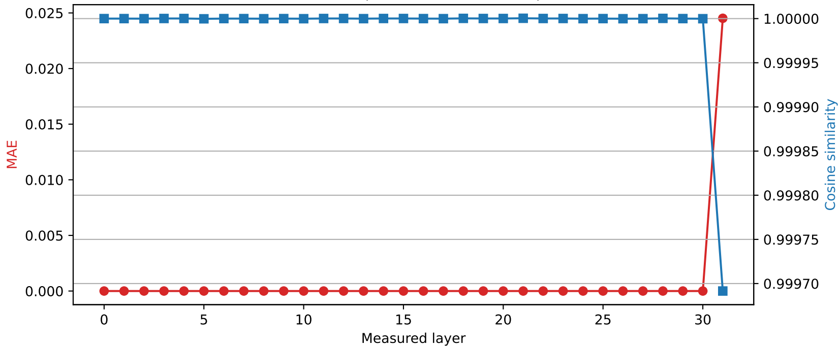
Mistral-7B-Instruct-v0.3 | Quantized layer 30 | float32 \rightarrow int8
