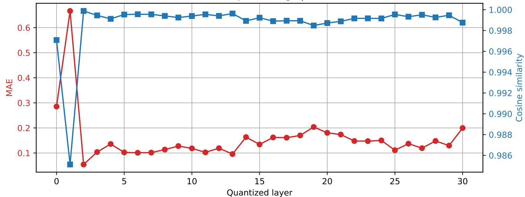
Mistral-7B-Instruct-v0.3 | Prompt 1 Final RMSNorm output damage | float32 → int8
